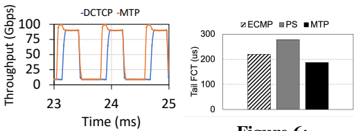
Figure 6: Load-and-request-aware load balancing
